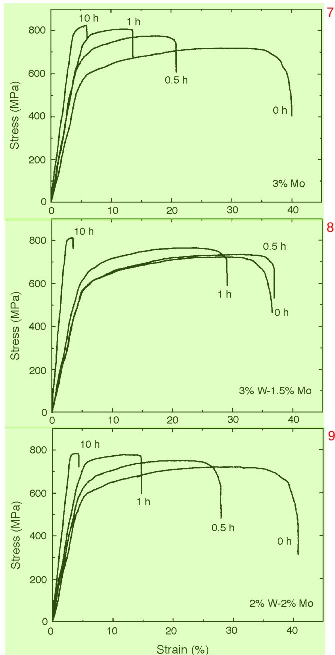
FIGURE 6. Effects of aging at 850°C on stress-vs-strain behavior of the designed alloys: 3% Mo, 3% W-1.5% Mo, and 2% W-2% Mo.
