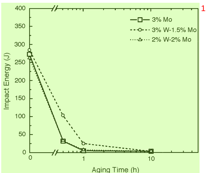
FIGURE 5. Effects of aging at 850°C on the Charpy impact toughness of the designed alloys: 3% Mo, 3% W-1.5% Mo, and 2% W-2% Mo.
