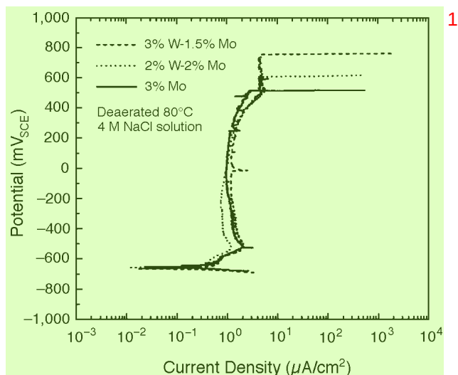
FIGURE 1. Effects of W substitution for Mo on anodic polarization responses in deaerated, 80°C, 4 M NaCl solution.
